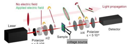
Figure 7: Free-space optics schematic.
